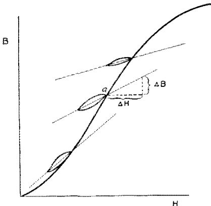
FIG. 2. EXPLANATORY DIAGRAM—INCREMENTAL PERMEABILITY CURVE
