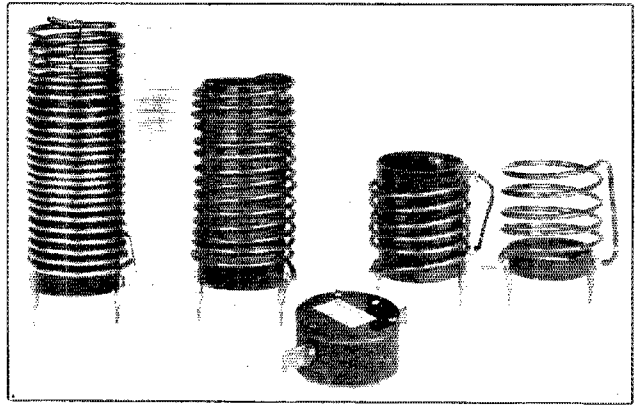
THE TUNING INDUCTANCES OF THE SET, ALL WOUND WITH NO. 8 BARE COPPER WIRE ON CARDWELL R.F. CHOKE FORMS, 1 \frac{1}{4} " IN DIAMETER
